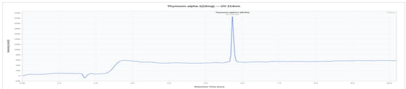
Thymosin Alpha-1 10mg - Lot 0826: UV Chromatogram
