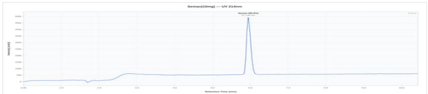
Semax 10mg - Lot 0826: UV Chromatogram
